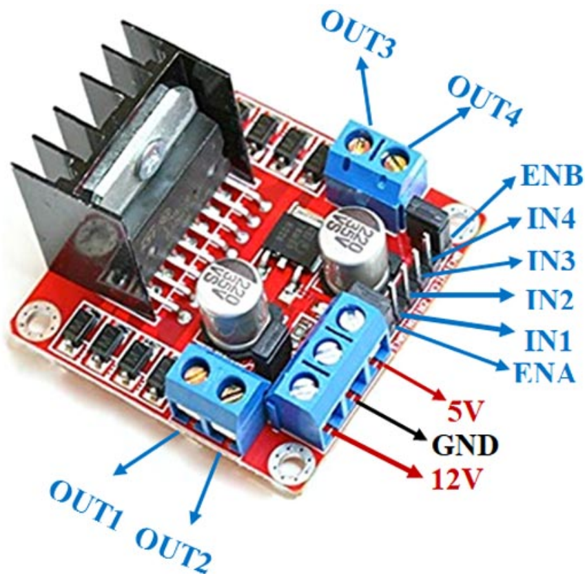
Fig. 3: L298N H bridge connections.
